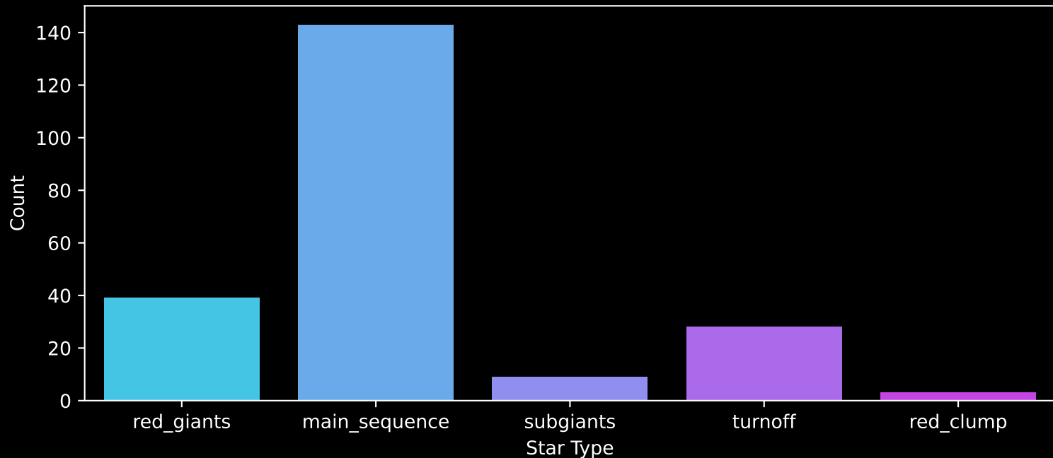
APOGEE DR17 Field: [K2_C14_250+51] Count plot of Star Type
