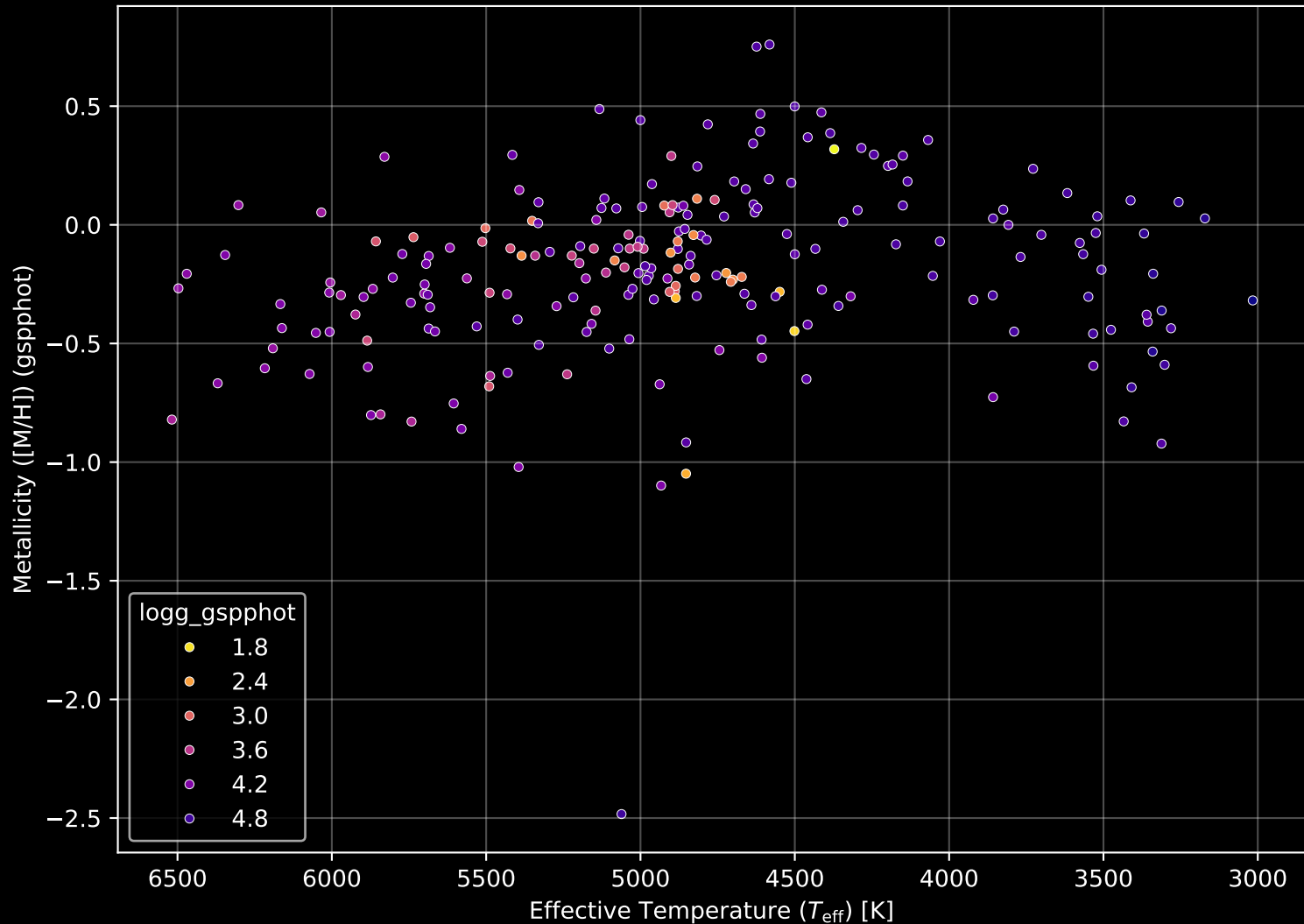
APOGEE DR17 Field: [K2_C14_250+51] Stellar Population Parameters (n= 222)
