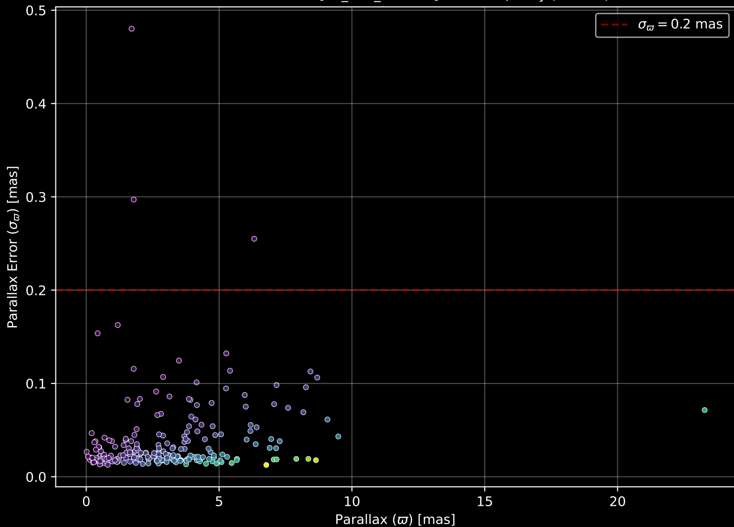
APOGEE DR17 Field: [K2_C14_250+51] Parallax Quality (n= 222)
