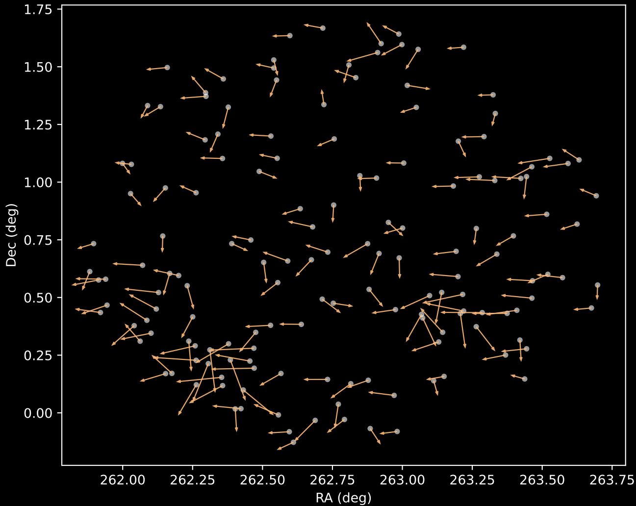
APOGEE DR17 Cluster 3 Proper Motion Vectors (n=155)
