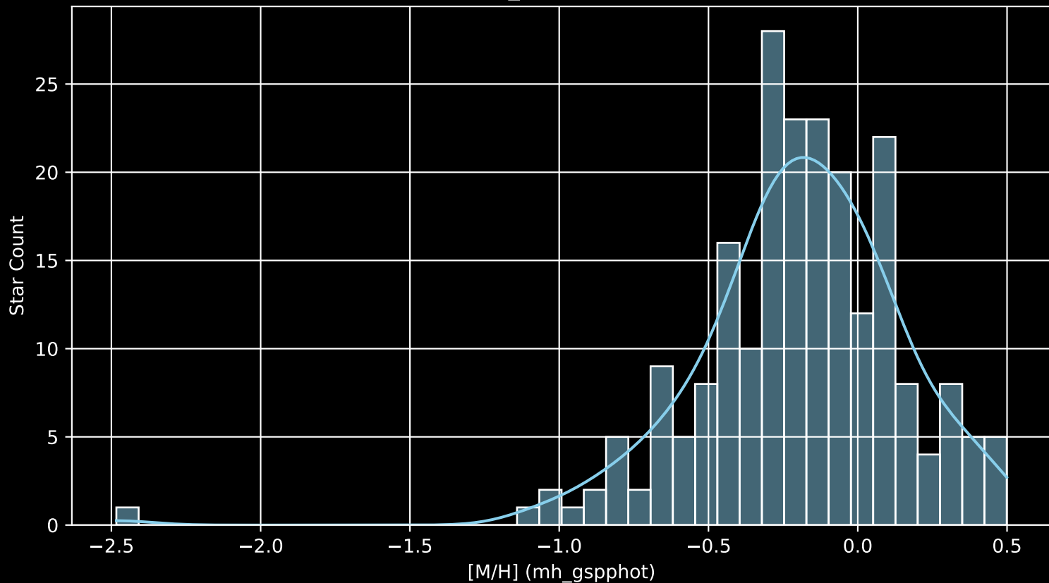
APOGEE DR17 Field: [K2_C14_250+51 [M/H] (mh_gspphot) (n= 220)
