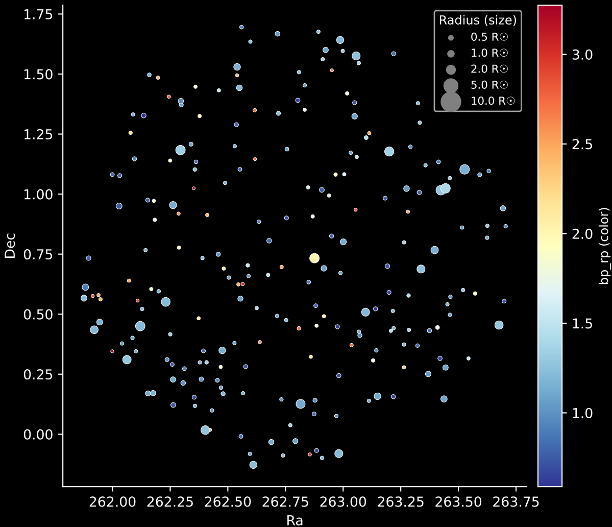
APOGEE DR17 Field: [K2_C14_250+51] Stars: 222
