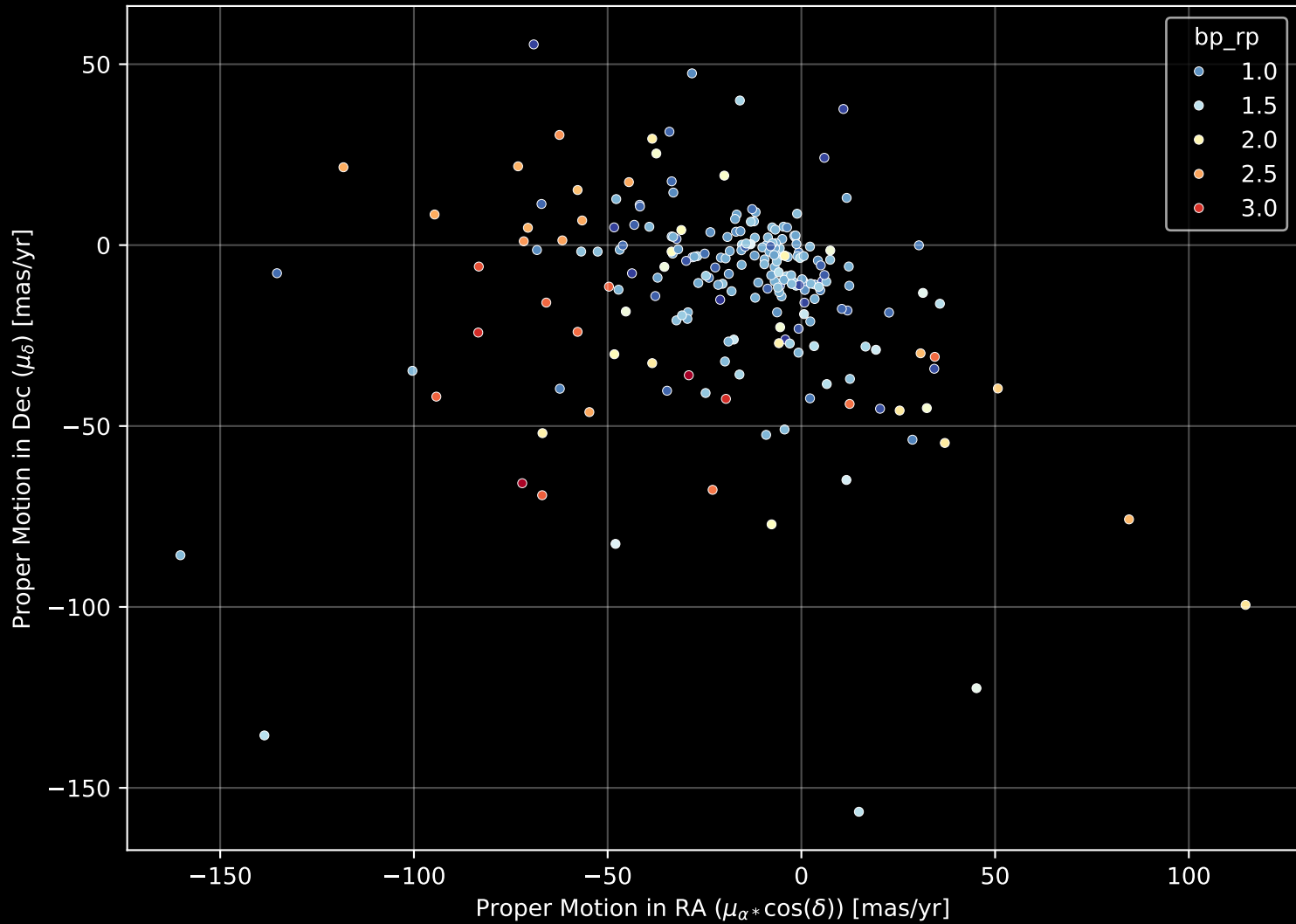
APOGEE DR17 Field: [K2_C14_250+51] Proper Motion Diagram (n= 222)
