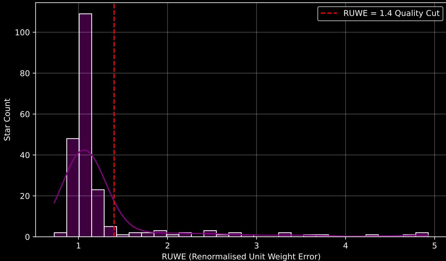
GAPOGEE DR17 Field [K2_C14_250+51] RUWE Distribution (n= 213)
